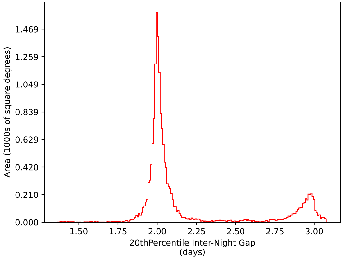
too_elab_r16_d2_ugrizy_v3.4_10yrs WFD i band: 20thPercentile Inter-Night Gap
