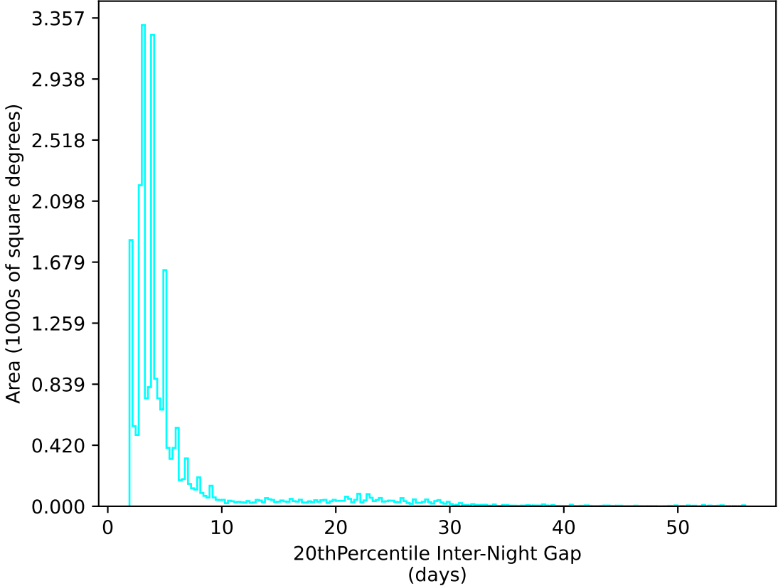
too_elab_r16_d2_ugrizy_v3.4_10yrs All sky u band: 20thPercentile Inter-Night Gap
