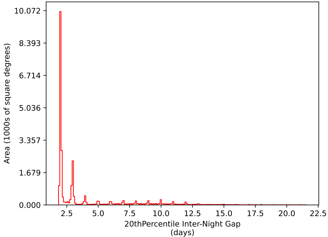
too_elab_r16_d2_ugrizy_v3.4_10yrs All sky i band: 20thPercentile Inter-Night Gap
