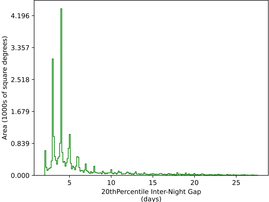
too_elab_r16_d2_ugrizy_v3.4_10yrs All sky g band: 20thPercentile Inter-Night Gap
