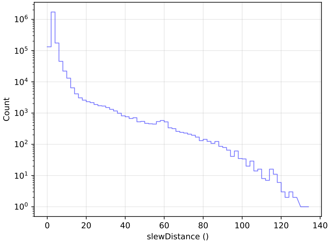
too_elab_r16_d2_ugrizy_v3.4_10yrs All visits: Slew Distance Histogram
