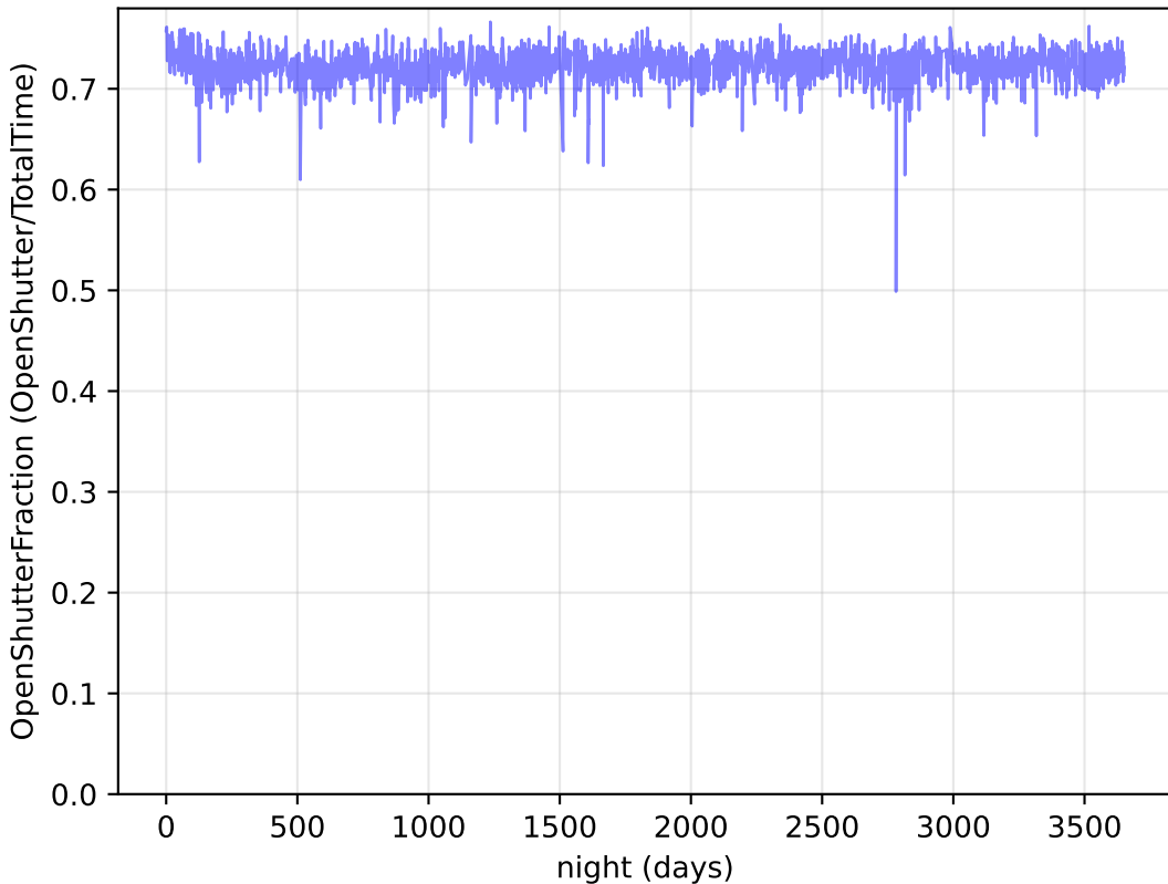
too_elab_r16_d2_ugrizy_v3.4_10yrs : OpenShutterFraction
