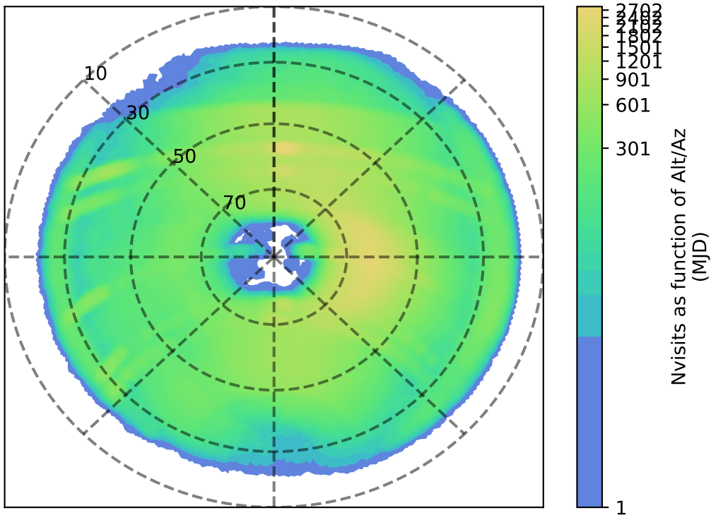
too_elab_r16_d2_ugrizy_v3.4_10yrs i: Nvisits as function of Alt/Az
