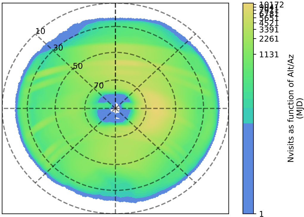
too_elab_r16_d2_ugrizy_v3.4_10yrs : Nvisits as function of Alt/Az
