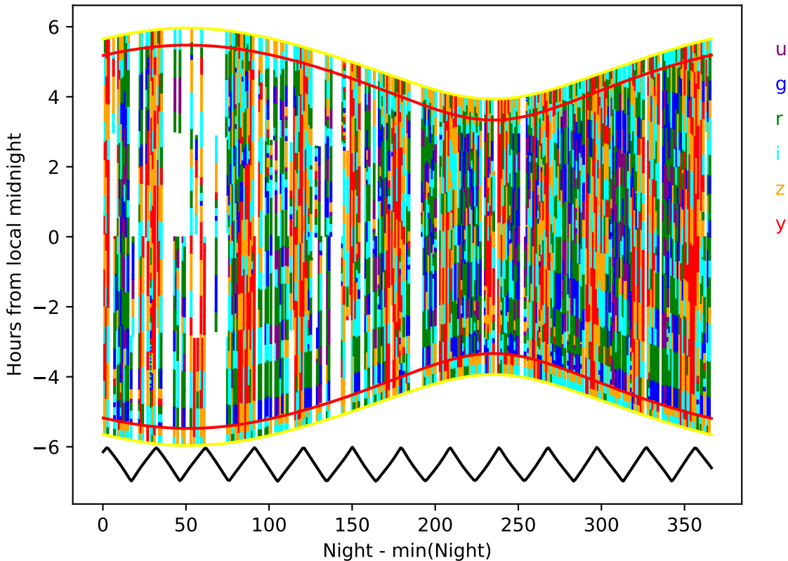
too_elab_r16_d2_ugrizy_v3.4_10yrs year 9-10: Hourglass
