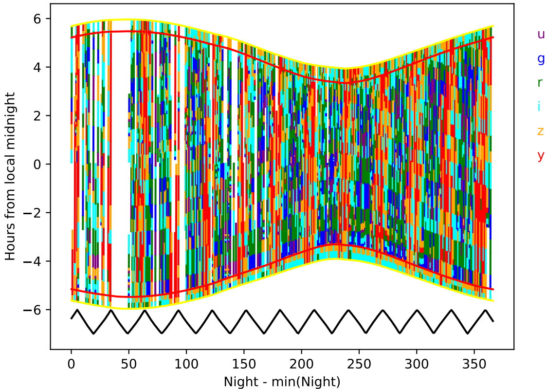
too_elab_r16_d2_ugrizy_v3.4_10yrs year 6-7: Hourglass
