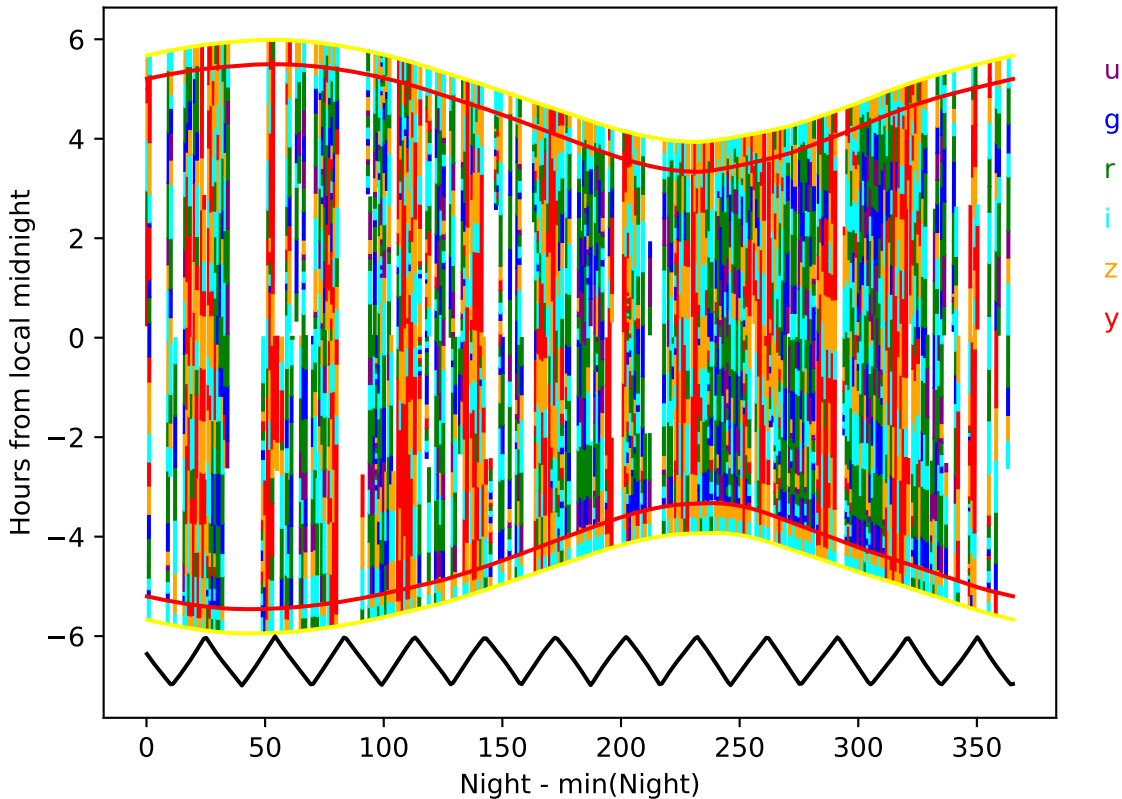
too_elab_r16_d2_ugrizy_v3.4_10yrs year 4-5: Hourglass
