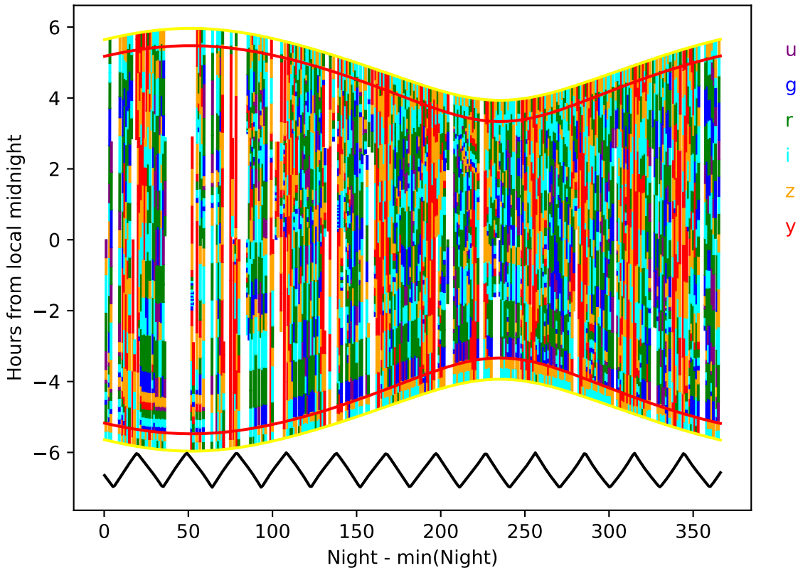
too_elab_r16_d2_ugrizy_v3.4_10yrs year 2-3: Hourglass
