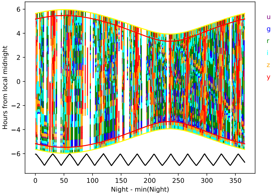
too_elab_r16_d2_ugrizy_v3.4_10yrs year 1-2: Hourglass
