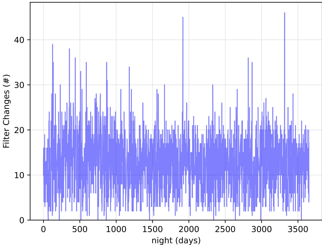
too_elab_r16_d2_ugrizy_v3.4_10yrs : Filter Changes
