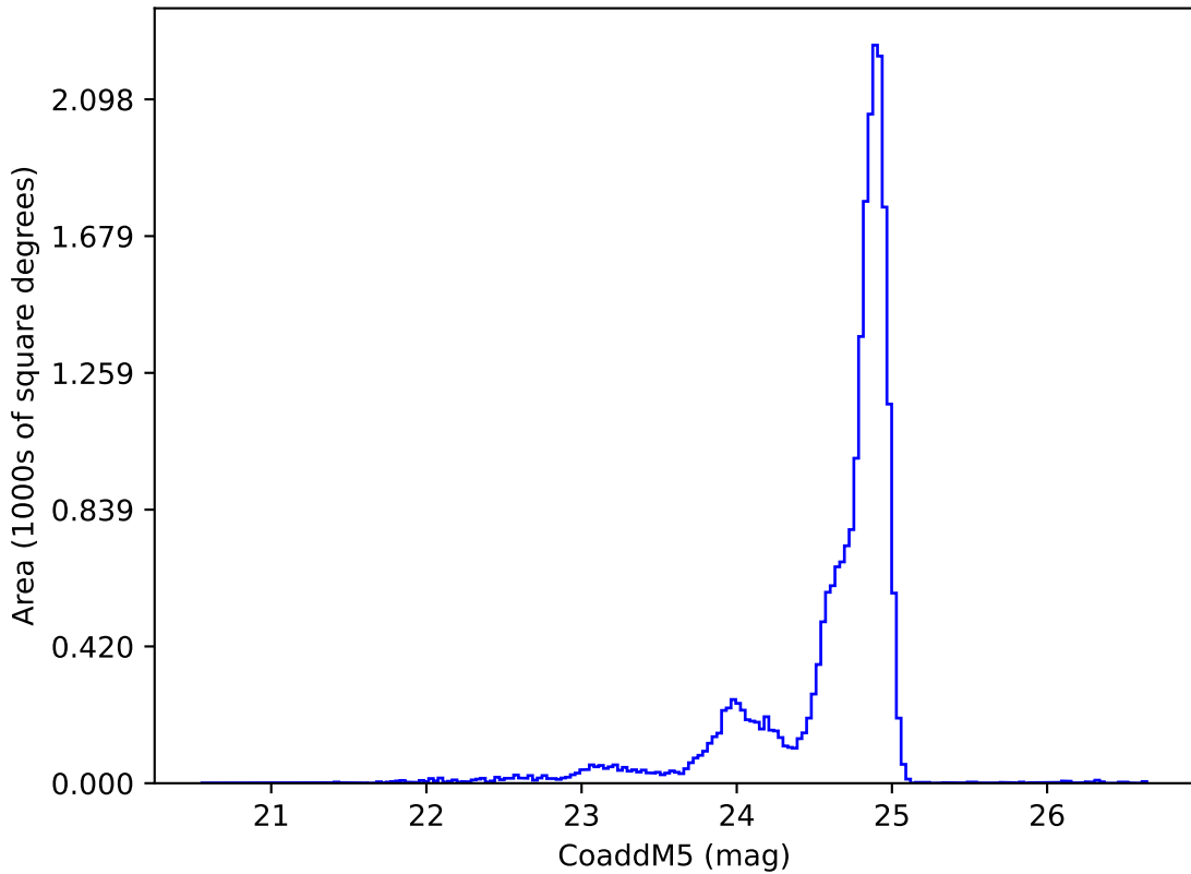
too_elab_r16_d2_ugrizy_v3.4_10yrs y: CoaddM5
