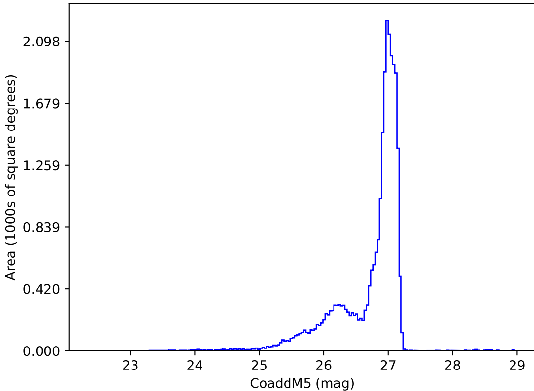
too_elab_r16_d2_ugrizy_v3.4_10yrs r: CoaddM5
