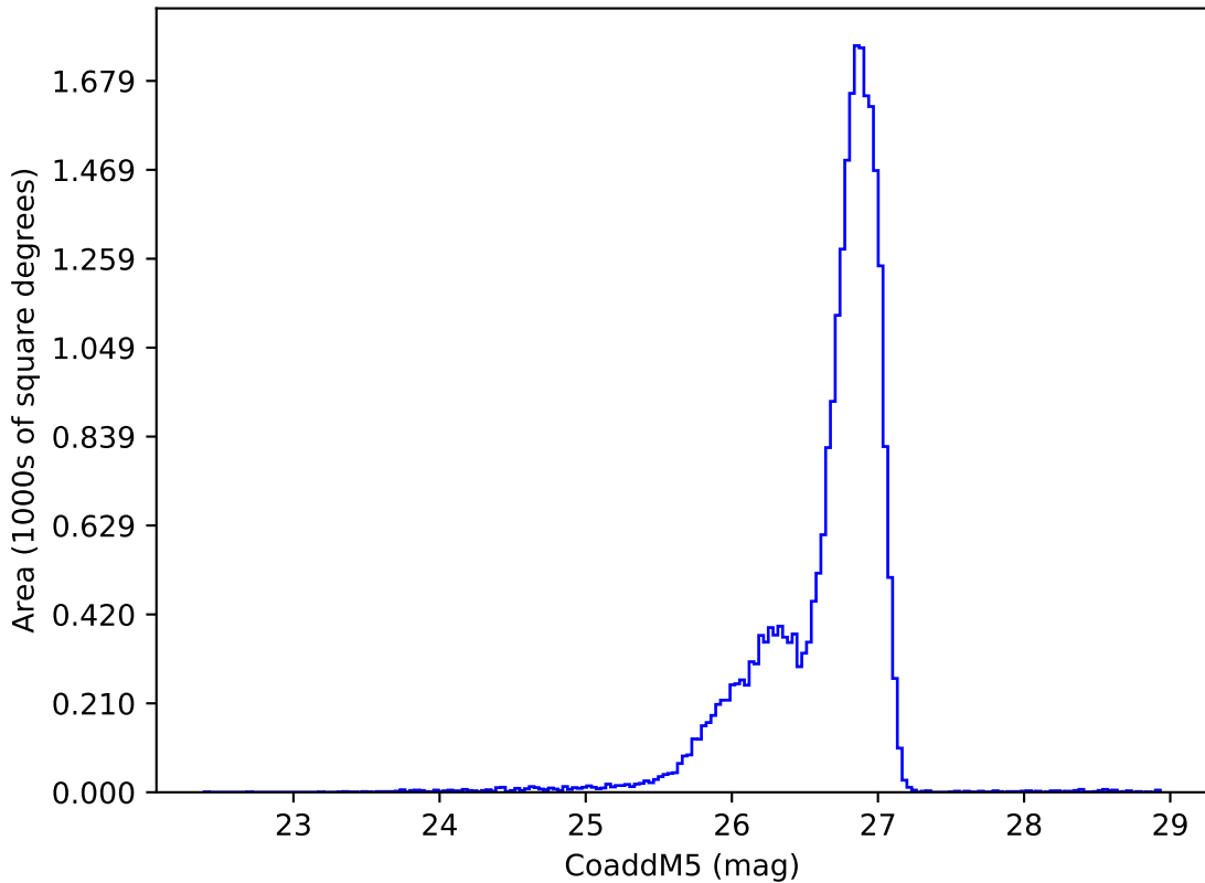
too_elab_r16_d2_ugrizy_v3.4_10yrs g: CoaddM5
