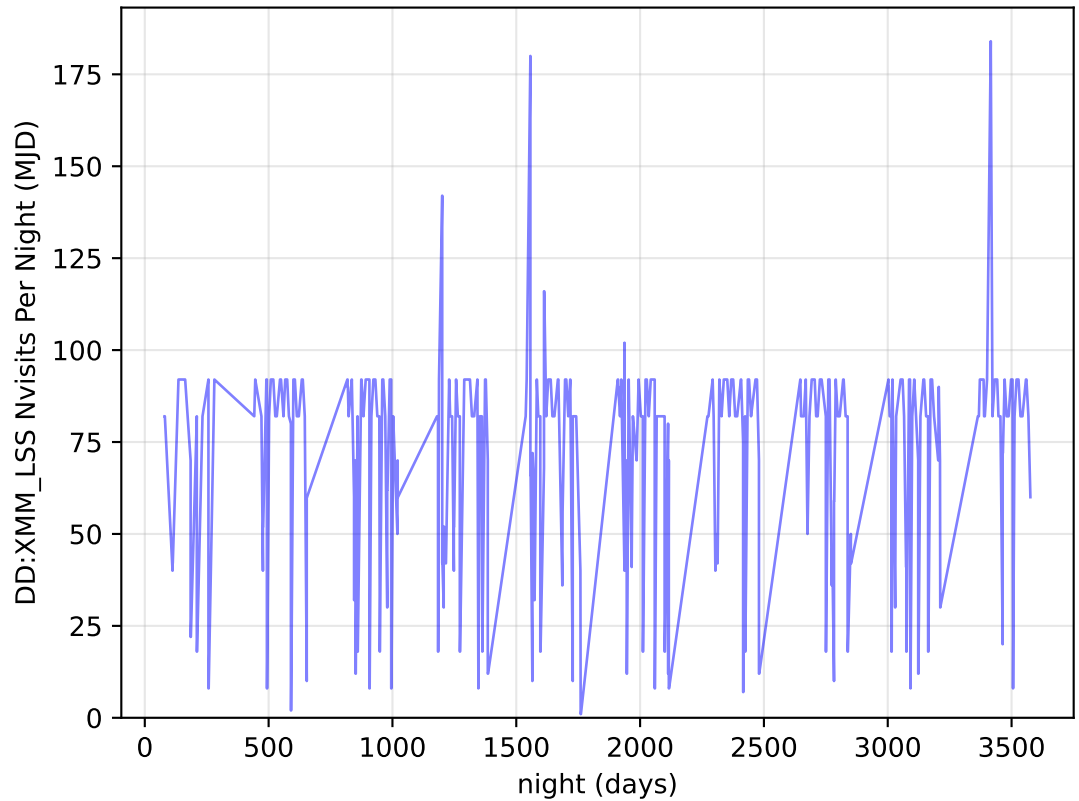
too_elab_r16_d2_ugrizy_v3.4_10yrs all bands: DD:XMM_LSS Nvisits Per Night
