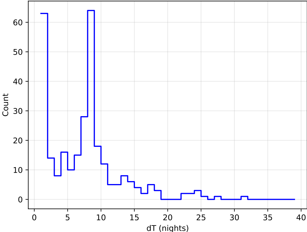
too_elab_r16_d2_ugrizy_v3.4_10yrs all bands: DD:XMM_LSS Delta Nights Histogram
