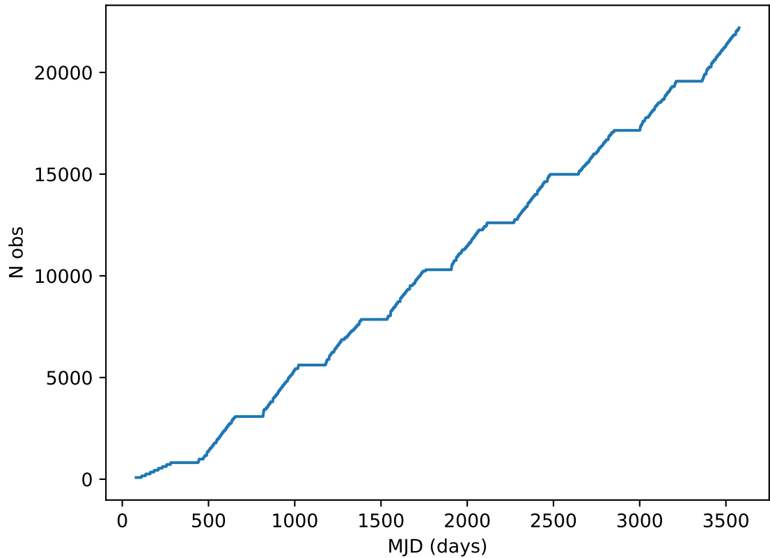
too_elab_r16_d2_ugrizy_v3.4_10yrs all bands: DD:XMM_LSS Cumulative NVisits
