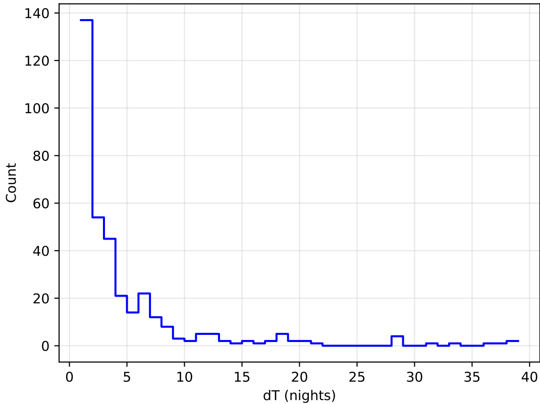
too_elab_r16_d2_ugrizy_v3.4_10yrs all bands: DD:WFD Delta Nights Histogram
