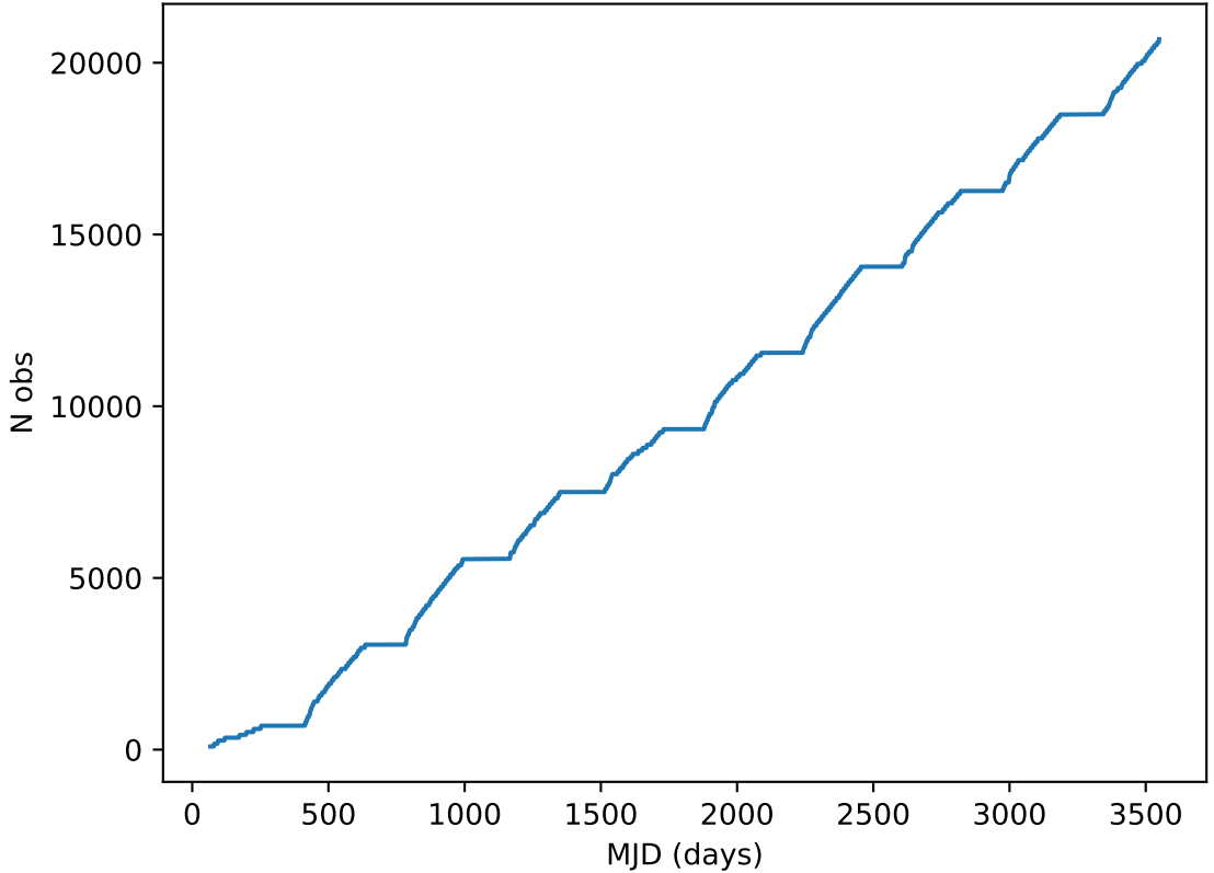
too_elab_r16_d2_ugrizy_v3.4_10yrs all bands: DD:ELAISS1 Cumulative NVisits
