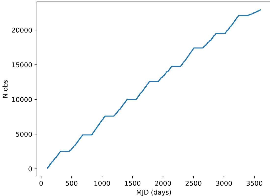
too_elab_r16_d2_ugrizy_v3.4_10yrs all bands: DD:EDFS Cumulative NVisits
