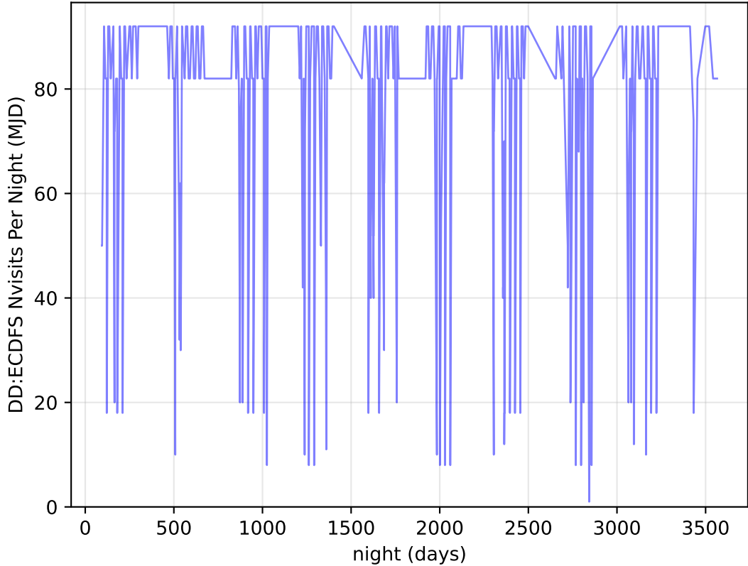
too_elab_r16_d2_ugrizy_v3.4_10yrs all bands: DD:ECDFS Nvisits Per Night
