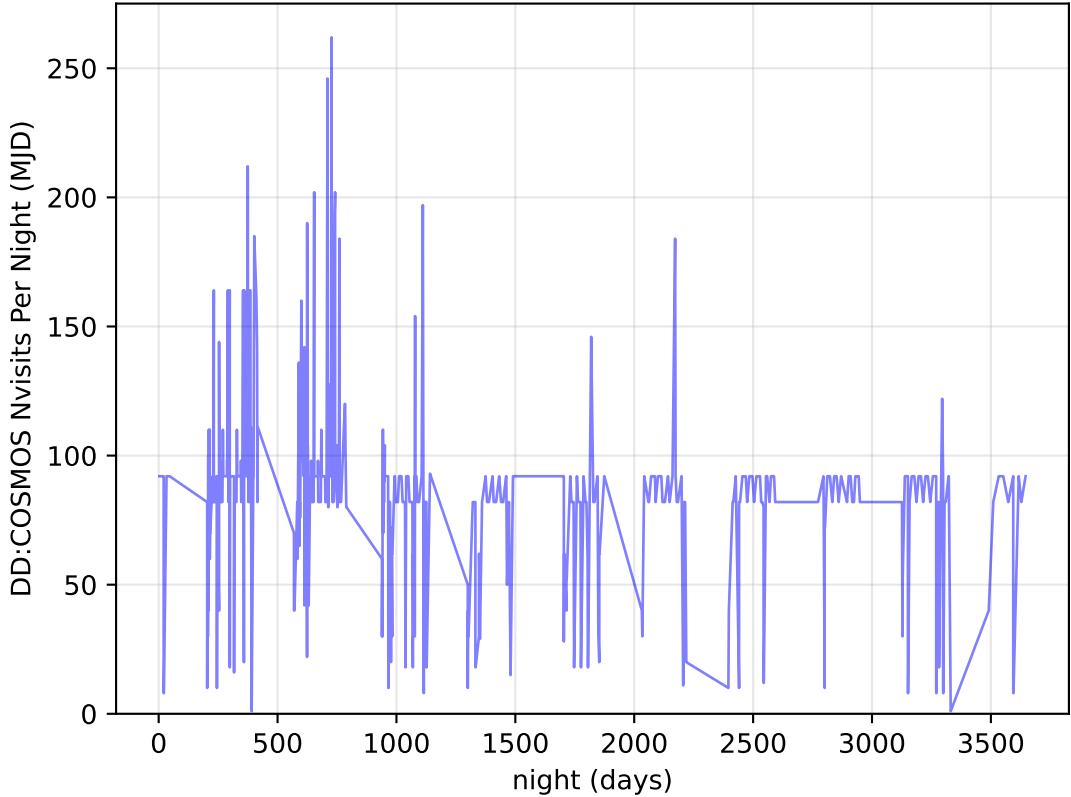
too_elab_r16_d2_ugrizy_v3.4_10yrs all bands: DD: COSMOS Nvisits Per Night
