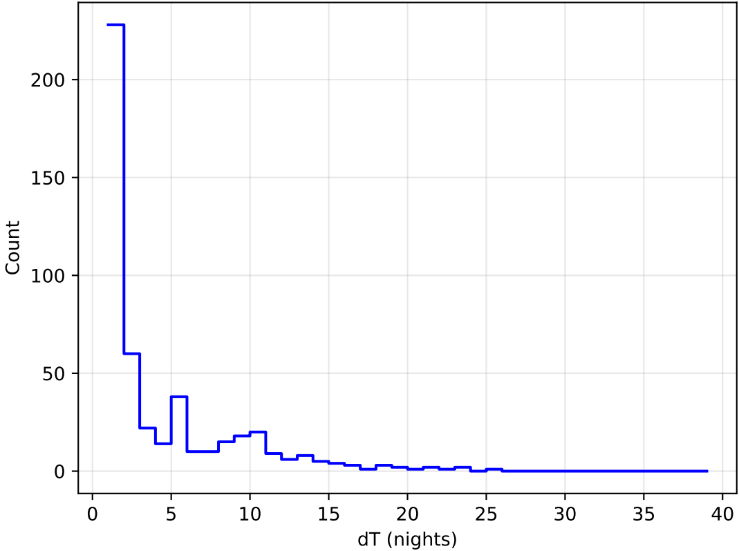
too_elab_r16_d2_ugrizy_v3.4_10yrs all bands: DD: COSMOS Delta Nights Histogram
