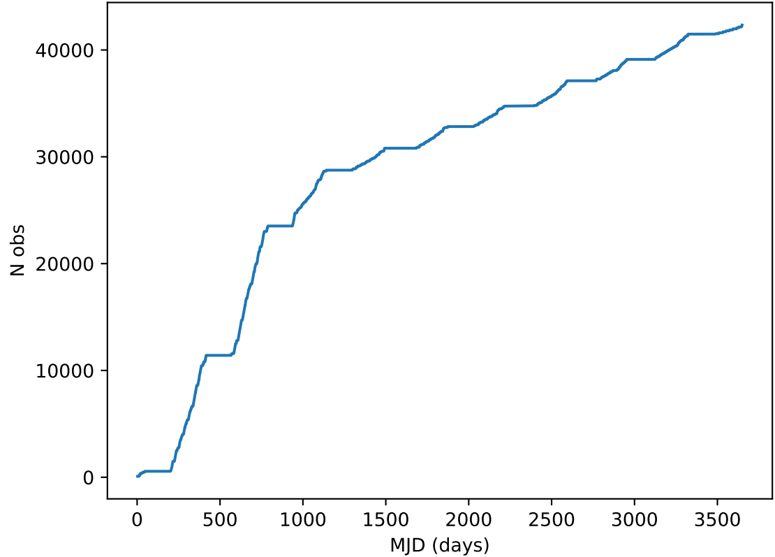
too_elab_r16_d2_ugrizy_v3.4_10yrs all bands: DD: COSMOS Cumulative NVisits
