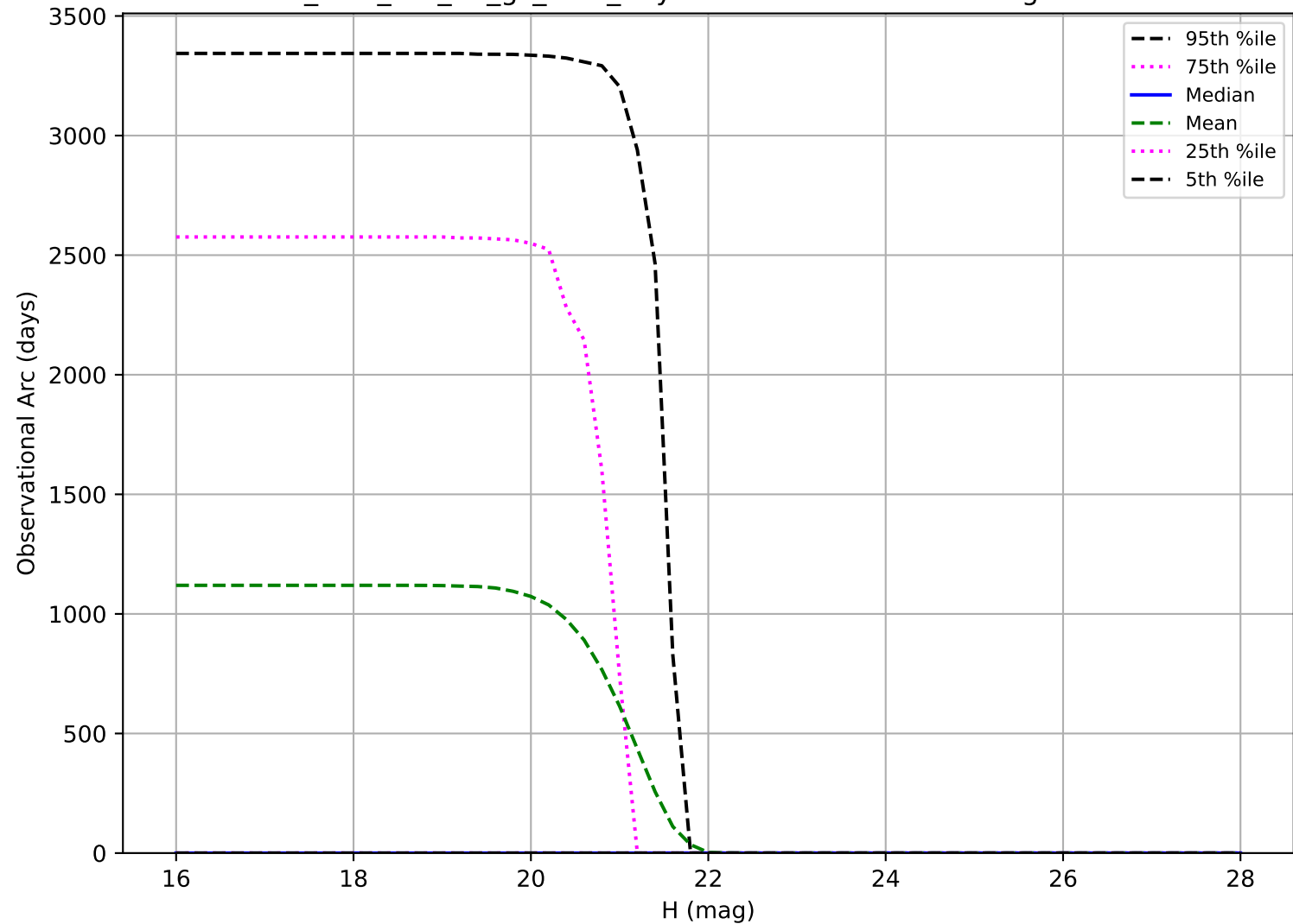
too_elab_r16_d2_gz_v3.4_10yrs: Observational Arc Length Vatira
