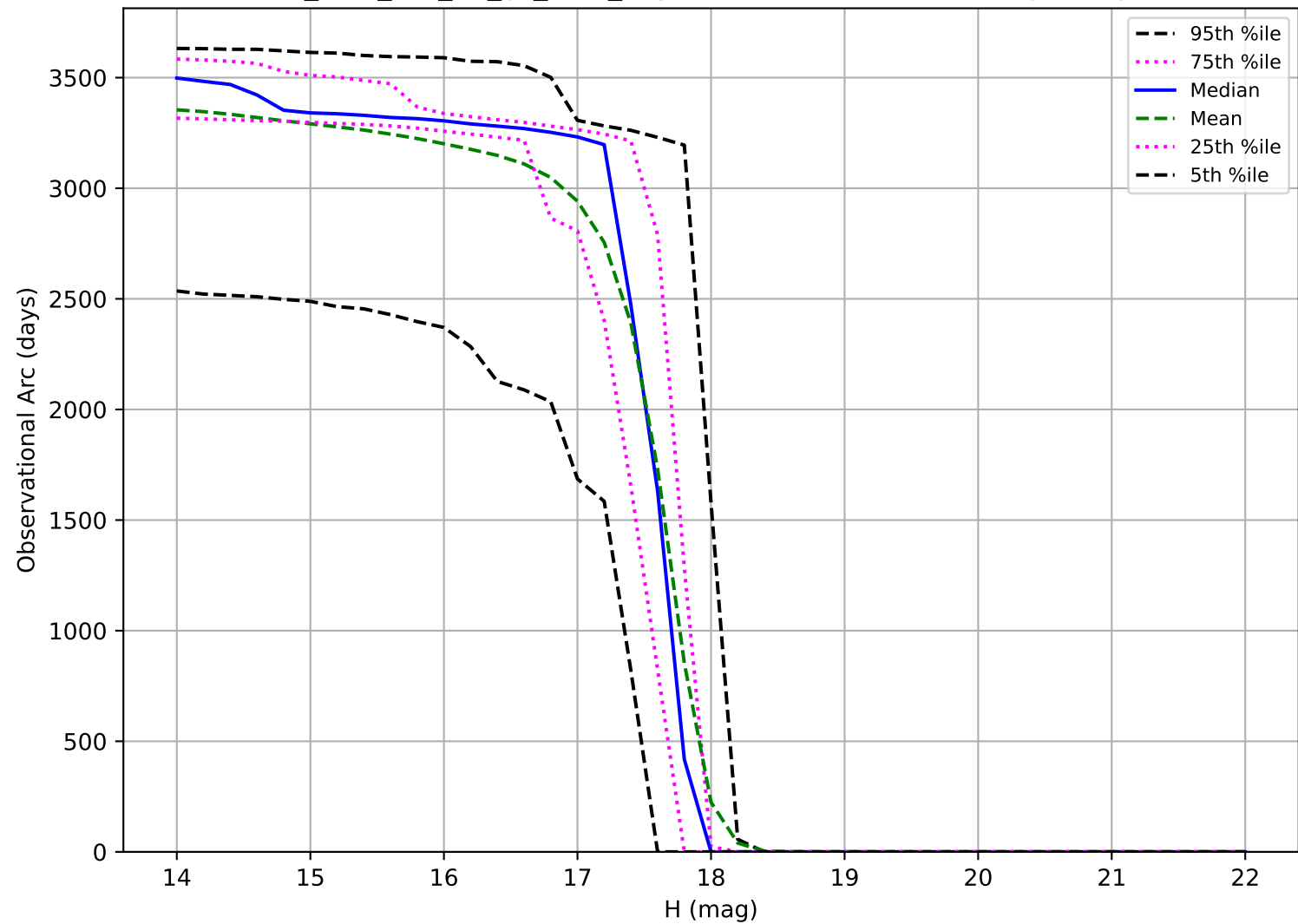
too_elab_r16_d2_gz_v3.4_10yrs: Observational Arc Length Trojan
