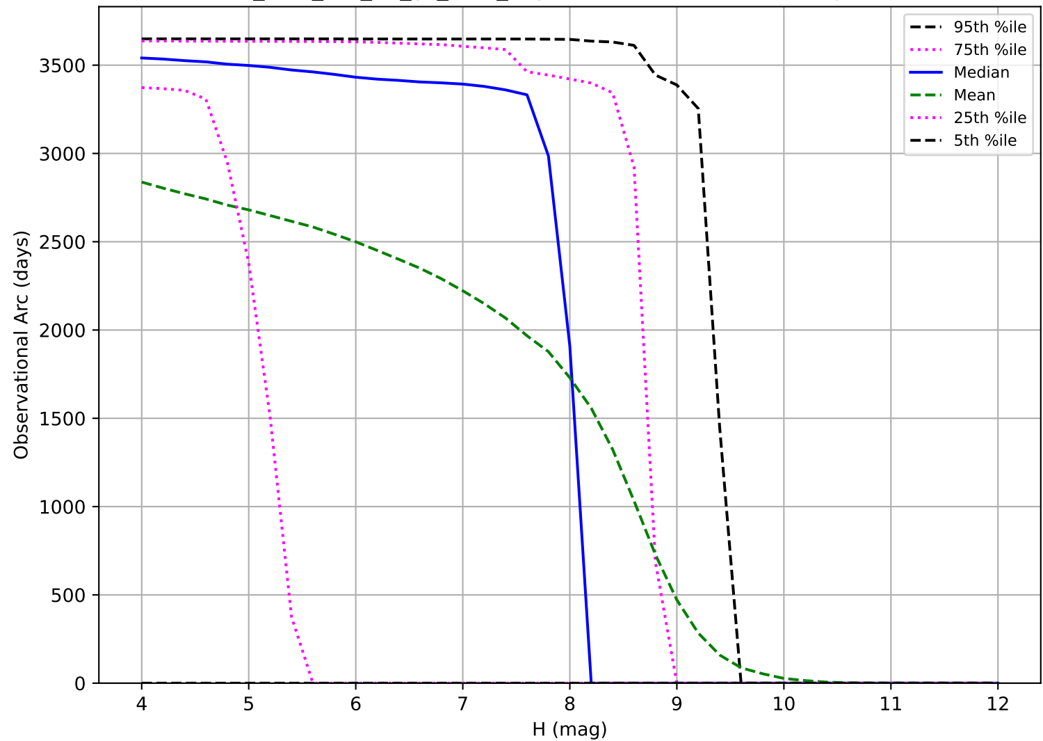
too_elab_r16_d2_gz_v3.4_10yrs: Observational Arc Length TNO
