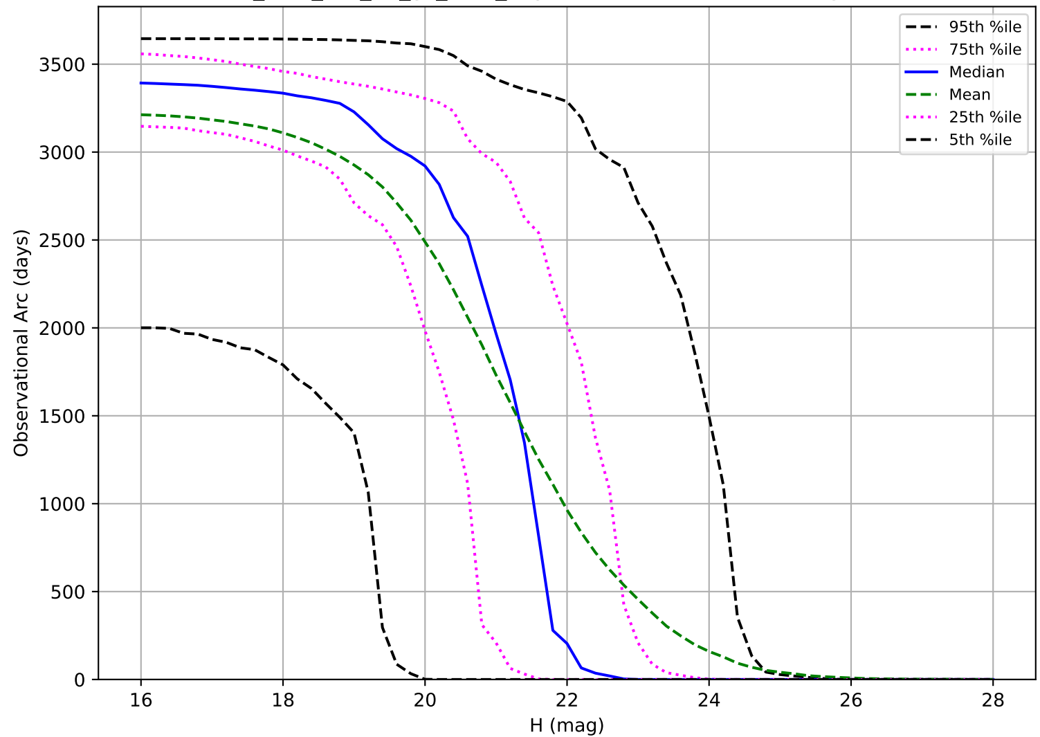
too_elab_r16_d2_gz_v3.4_10yrs: Observational Arc Length PHA
