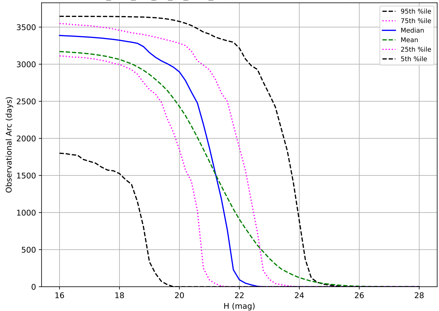
too_elab_r16_d2_gz_v3.4_10yrs: Observational Arc Length NEO
