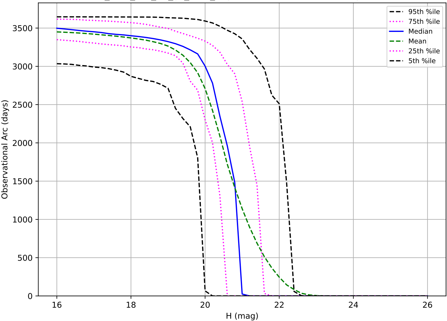
too_elab_r16_d2_gz_v3.4_10yrs: Observational Arc Length MBA
