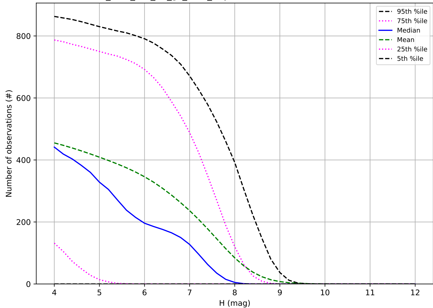
too_elab_r16_d2_gz_v3.4_10yrs: Number of observations TNO
