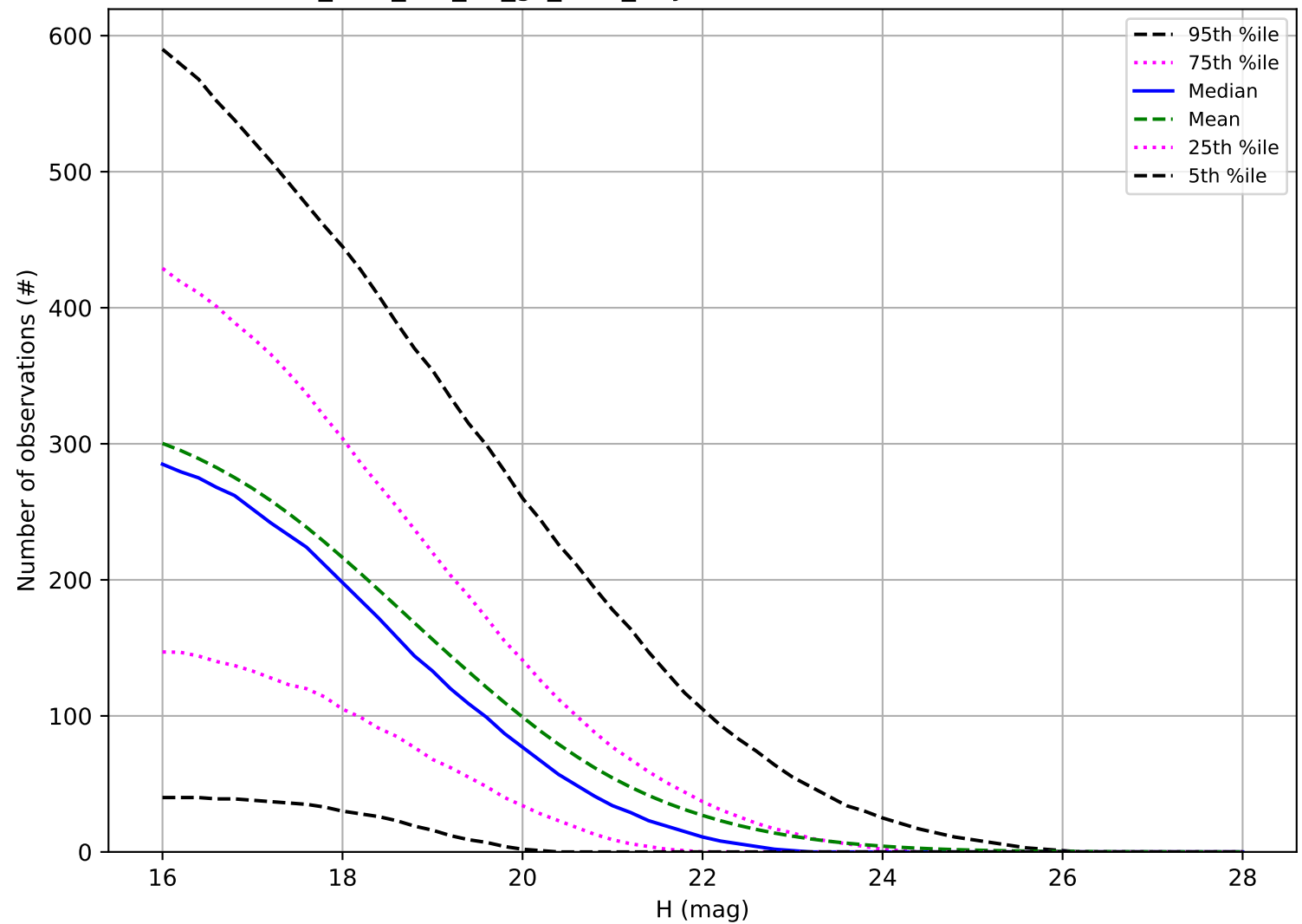
too_elab_r16_d2_gz_v3.4_10yrs: Number of observations PHA
