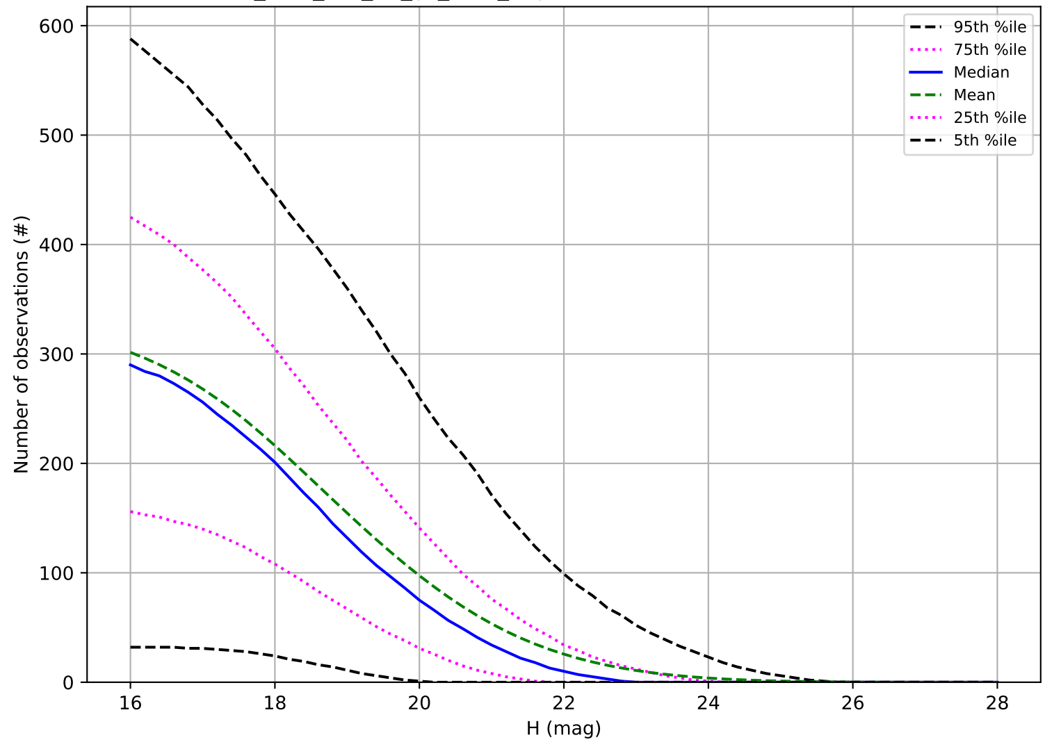
too_elab_r16_d2_gz_v3.4_10yrs: Number of observations NEO
