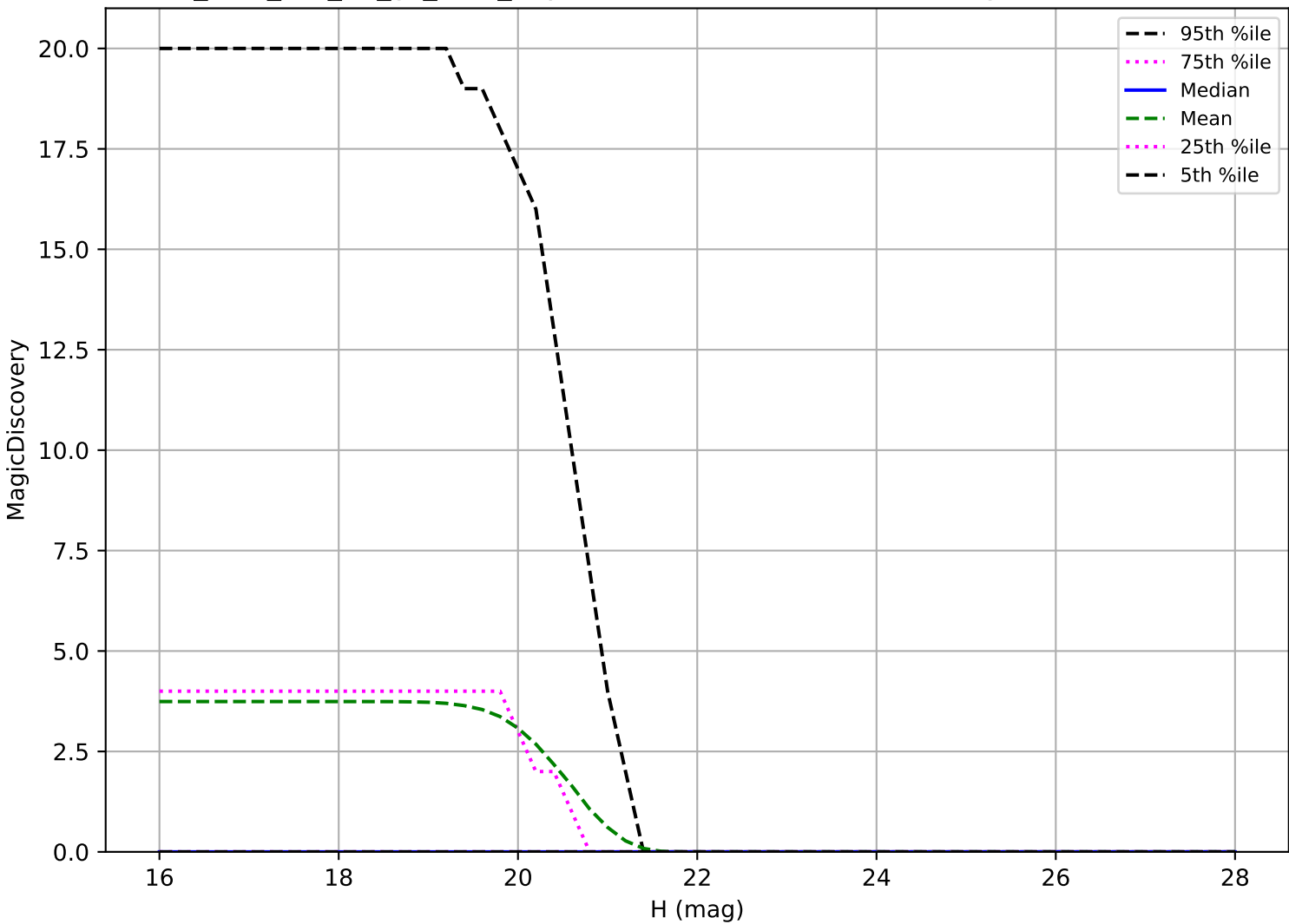
too_elab_r16_d2_gz_v3.4_10yrs: Vatra 6 detections in 60 nights detection loss
