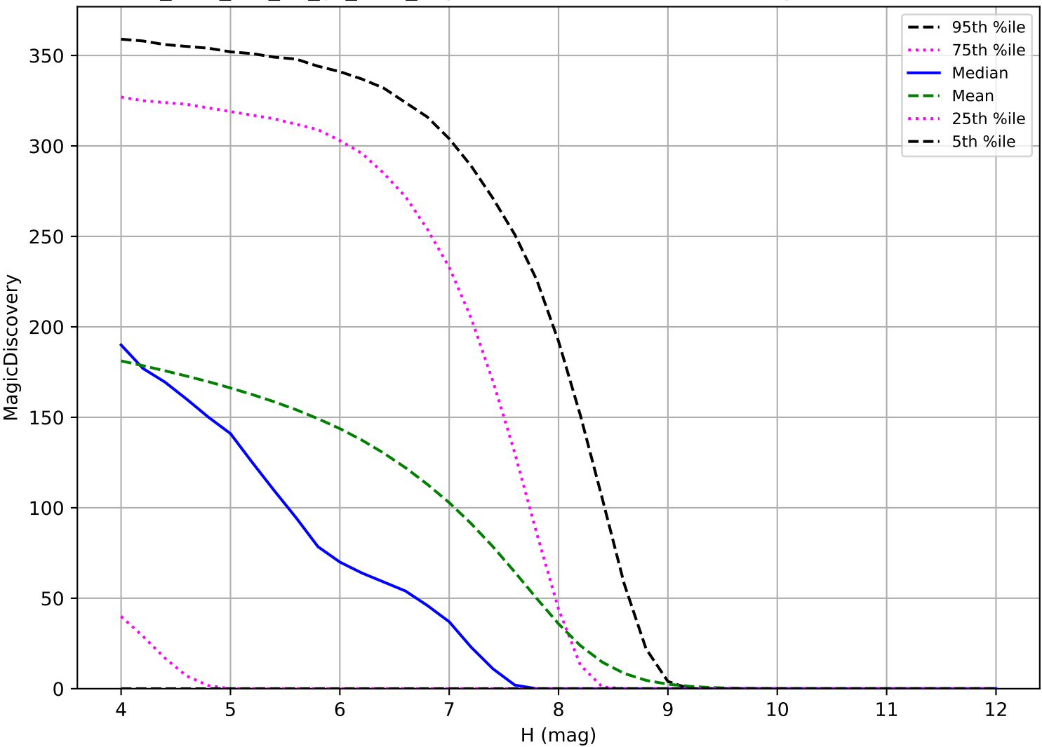
too_elab_r16_d2_gz_v3.4_10yrs: TNO 6 detections in 60 nights detection loss
