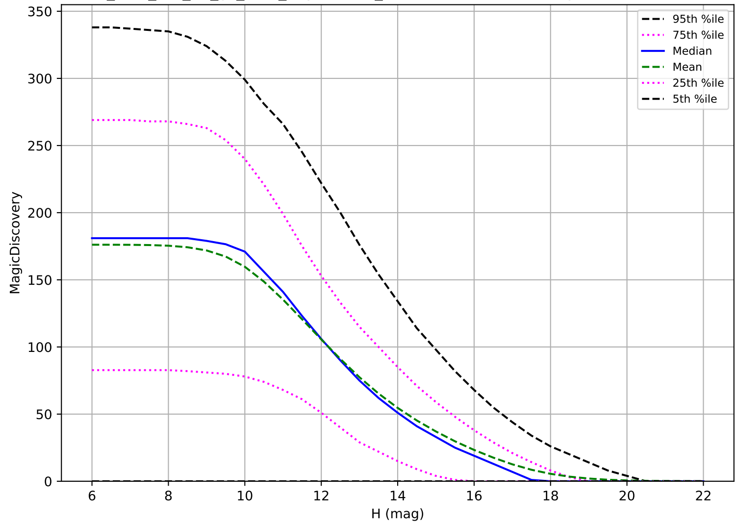
too_elab_r16_d2_gz_v3.4_10yrs: OCC_r5 6 detections in 60 nights detection loss
