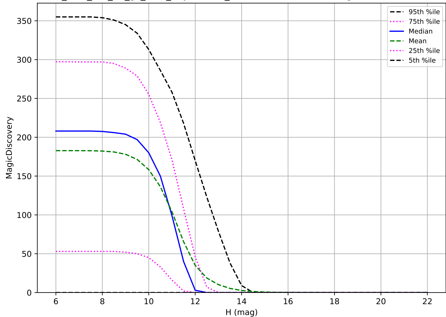
too_elab_r16_d2_gz_v3.4_10yrs: OCC_r20 6 detections in 60 nights detection loss
