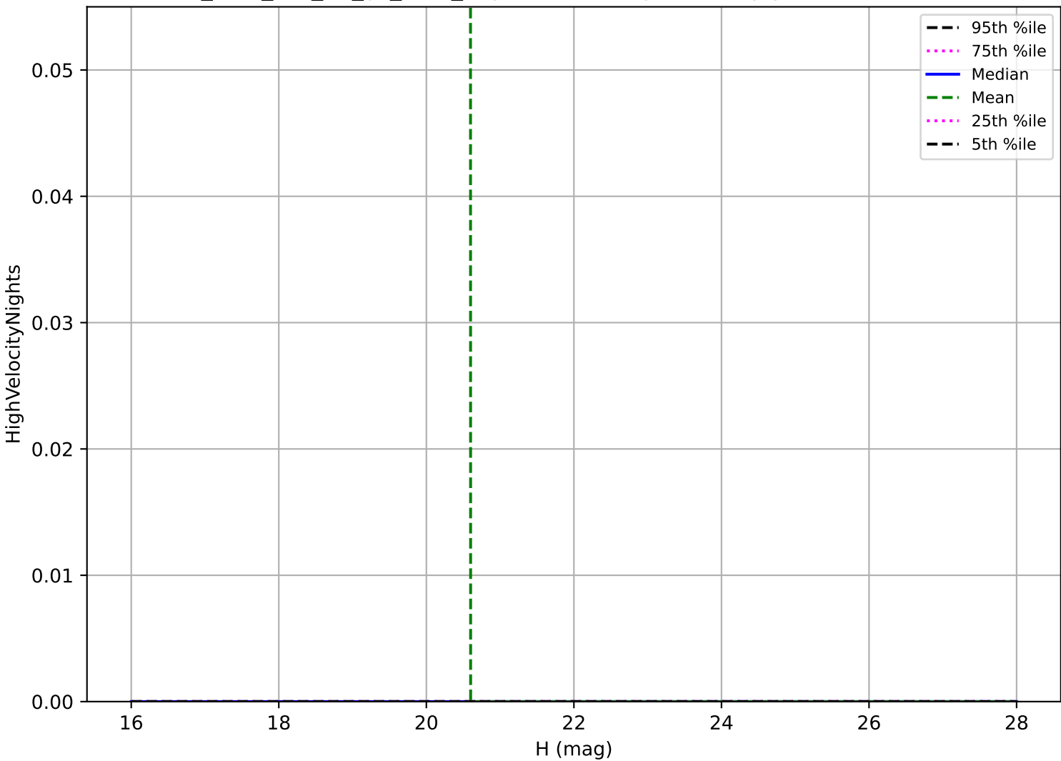
too_elab_r16_d2_gz_v3.4_10yrs: Vatira High velocity pair detection loss
