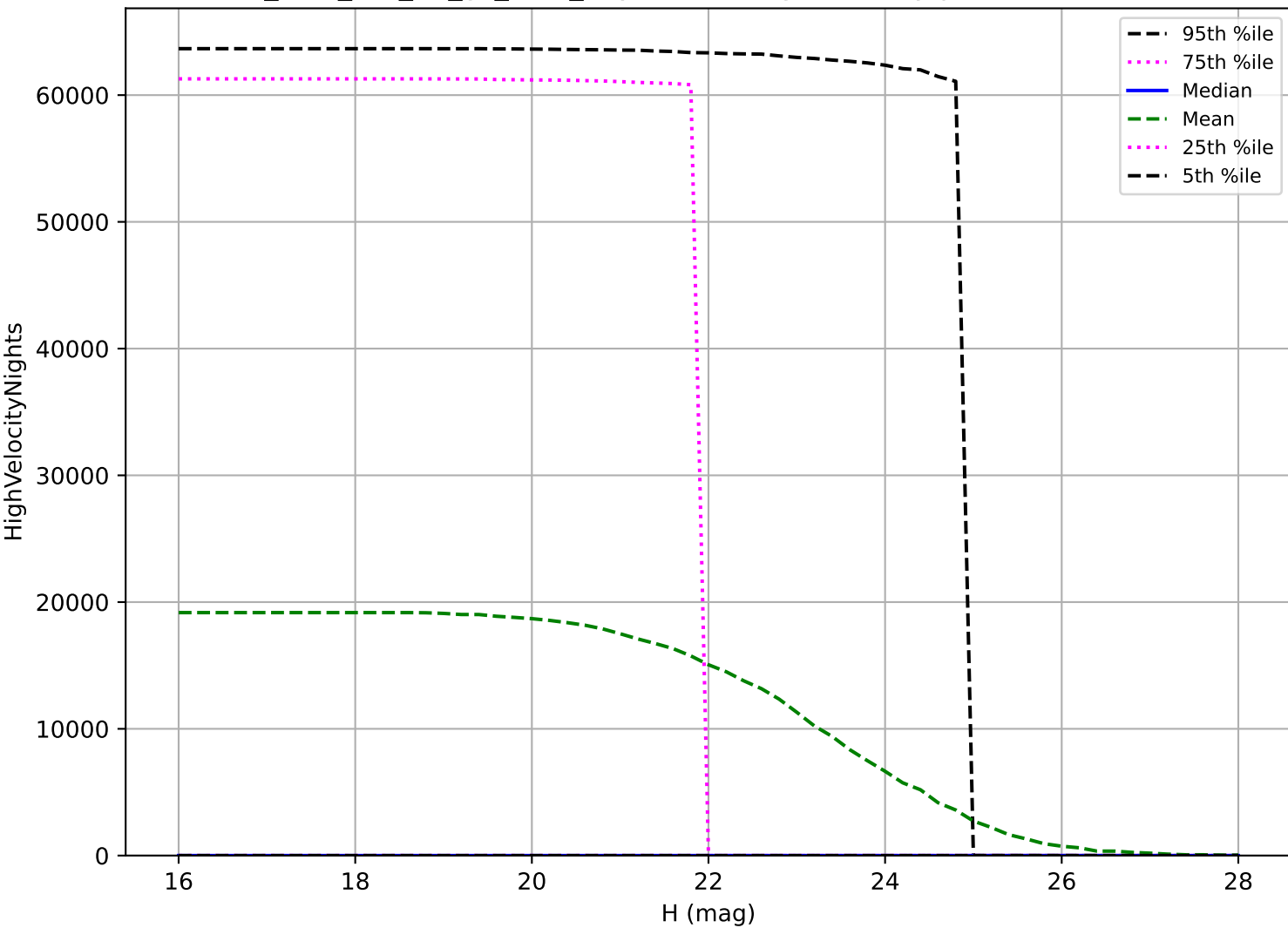
too_elab_r16_d2_gz_v3.4_10yrs: NEO High velocity pair detection loss
