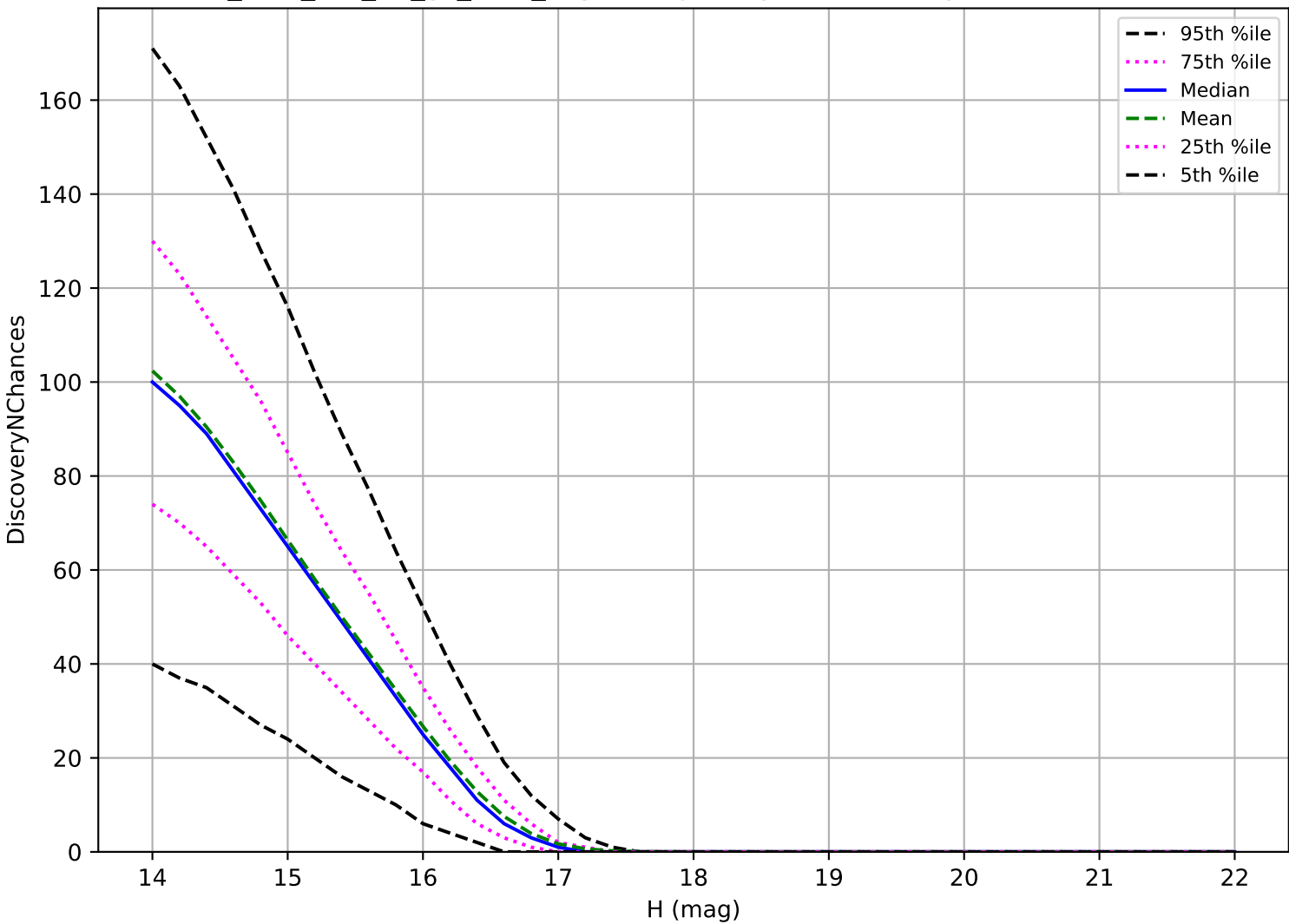
too_elab_r16_d2_gz_v3.4_10yrs: Trojan 3 pairs in 15 nights detection loss
