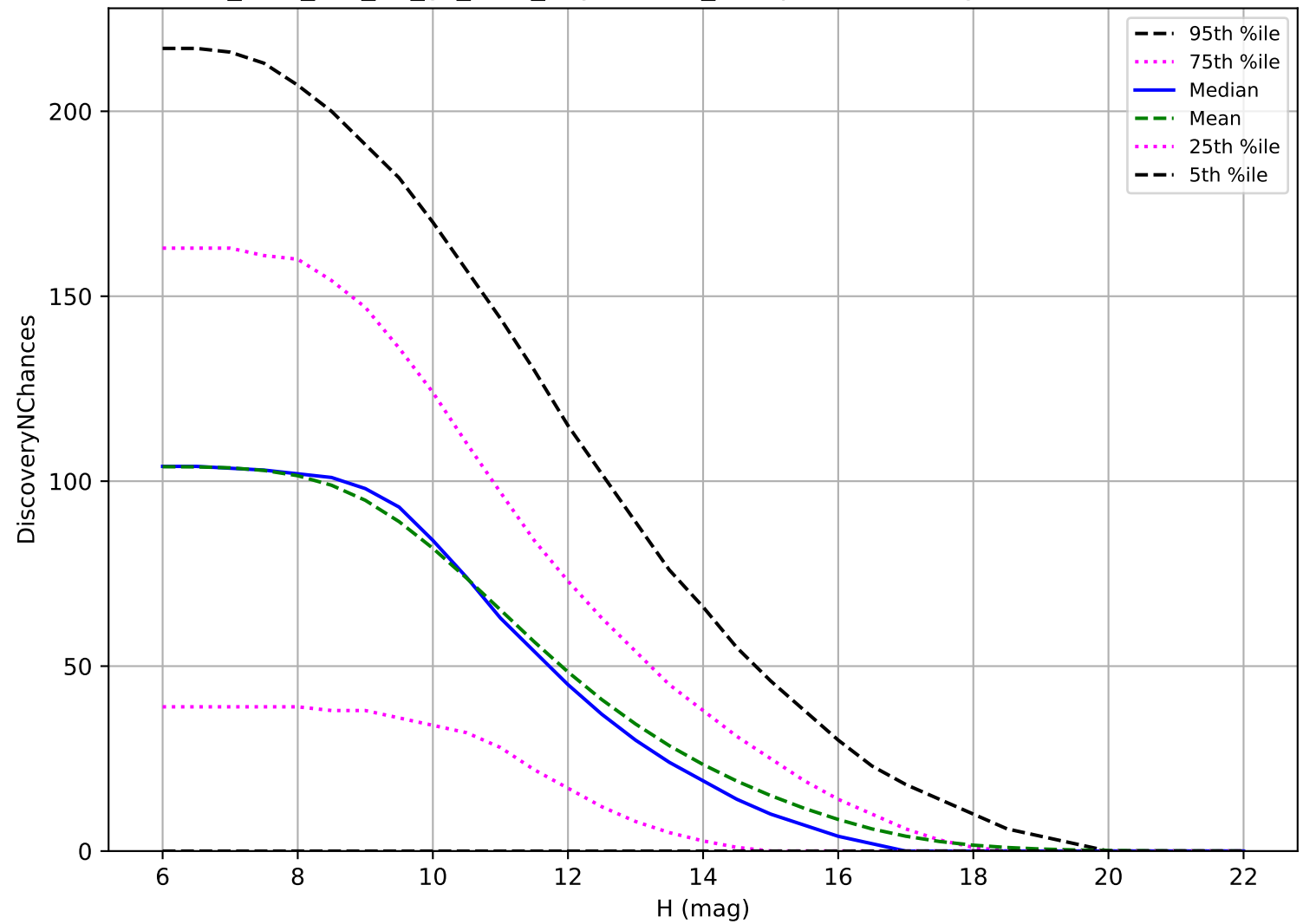
too_elab_r16_d2_gz_v3.4_10yrs: OCC_r5 3 pairs in 15 nights detection loss
