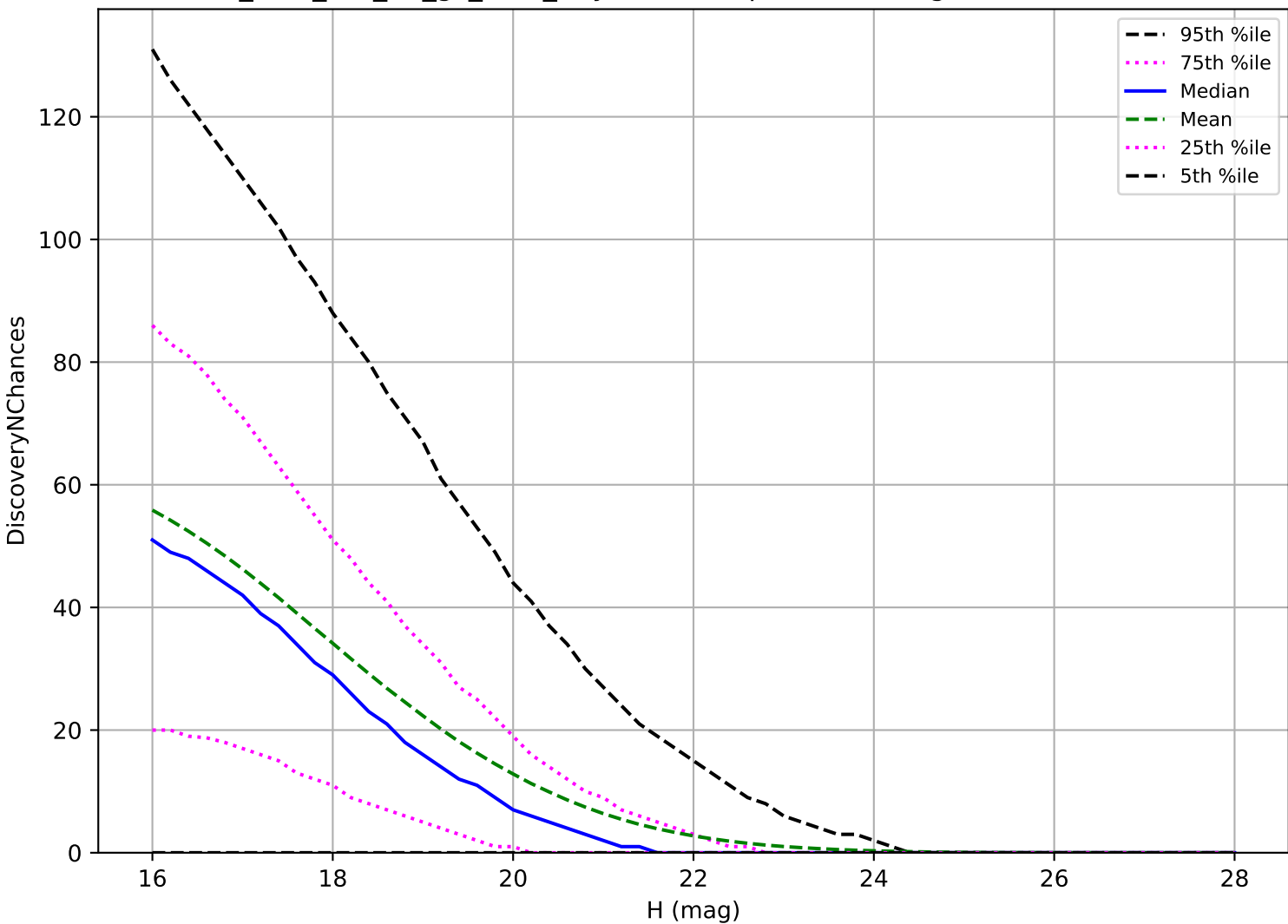
too_elab_r16_d2_gz_v3.4_10yrs: NEO 3 pairs in 15 nights detection loss
