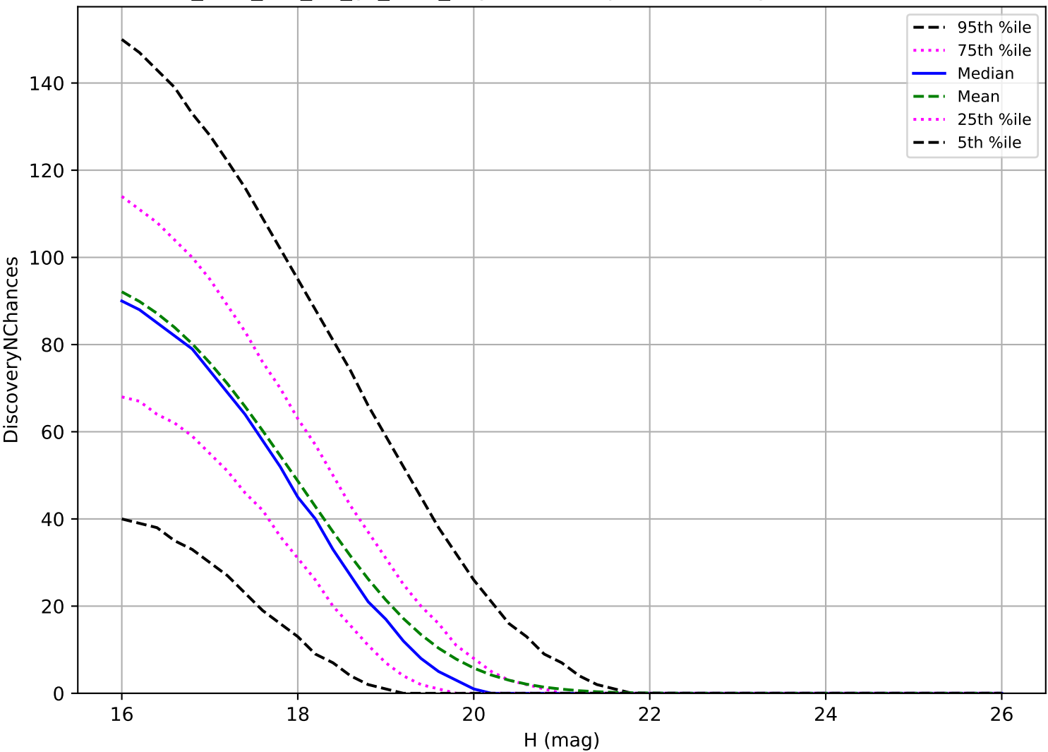
too_elab_r16_d2_gz_v3.4_10yrs: MBA 3 pairs in 15 nights detection loss
