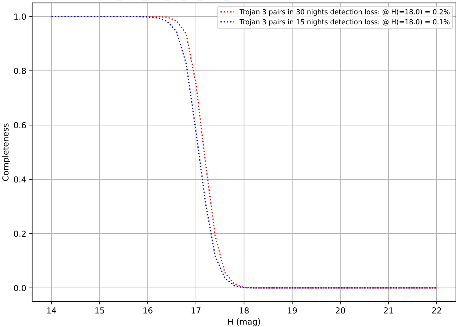
too_elab_r16_d2_gz_v3.4_10yrs: DifferentialCompleteness
