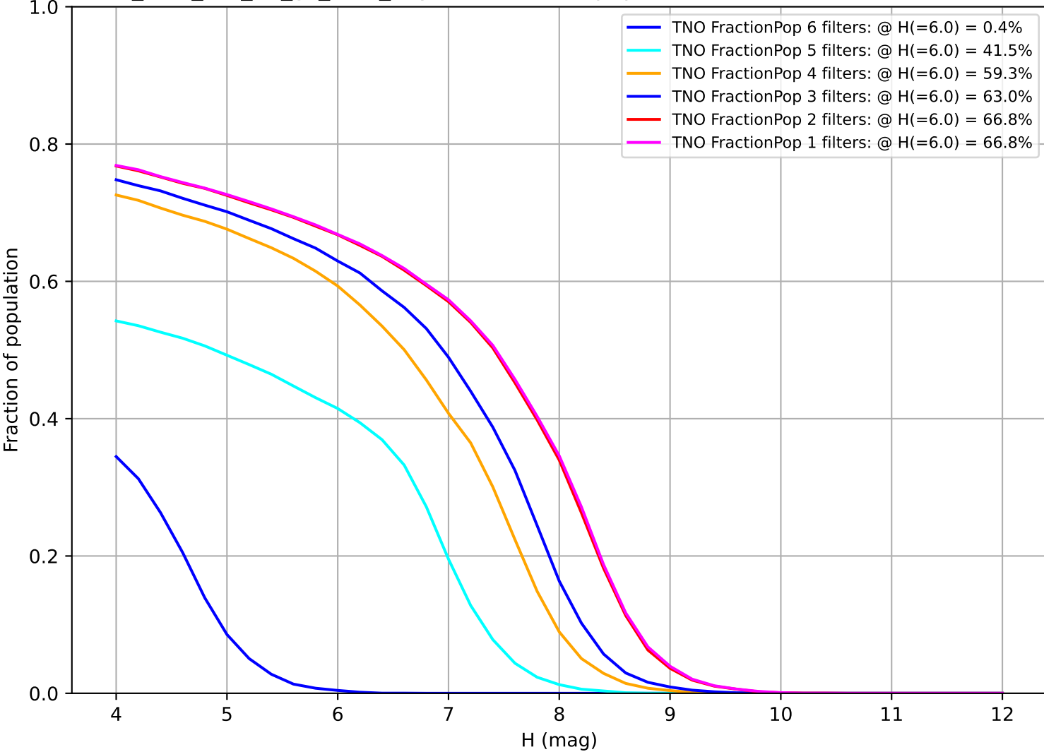
too_elab_r16_d2_gz_v3.4_10yrs: Fraction of population with colors in X filters TNO
