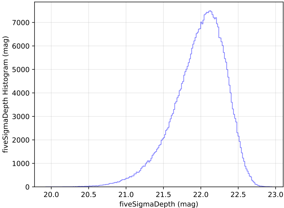
too_elab_r16_d2_gz_v3.4_10yrs y: fiveSigmaDepth Histogram
