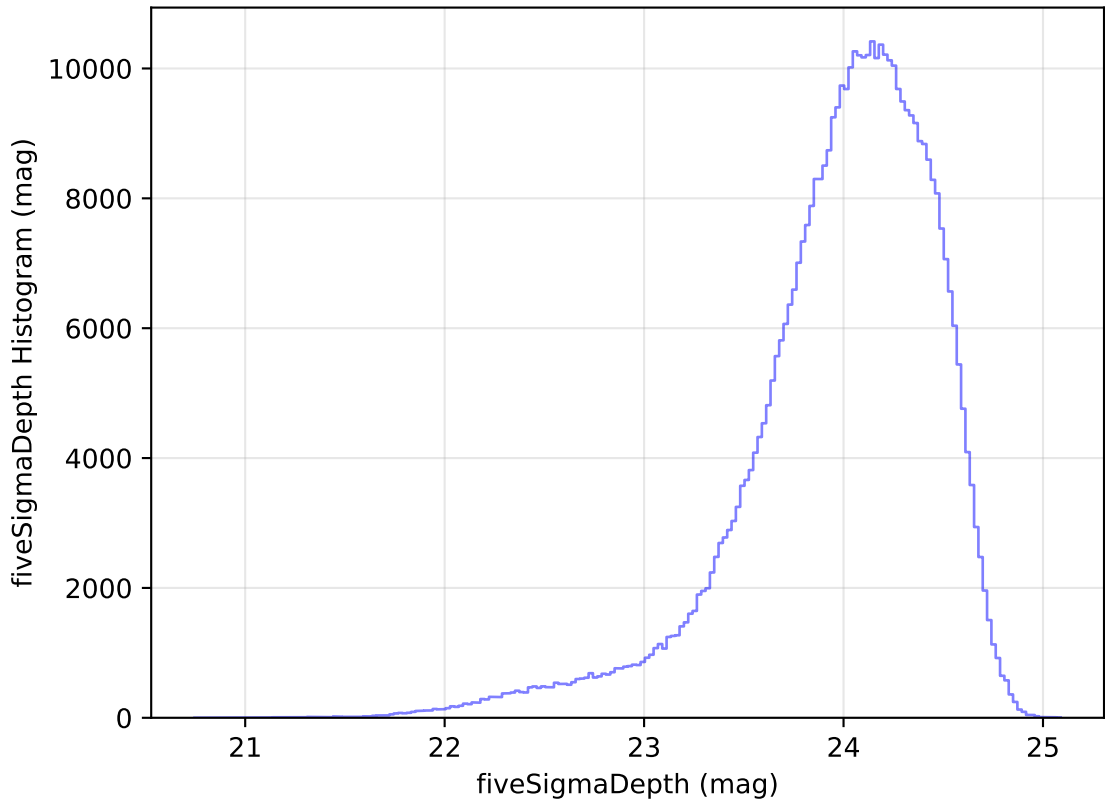
too_elab_r16_d2_gz_v3.4_10yrs r: fiveSigmaDepth Histogram
